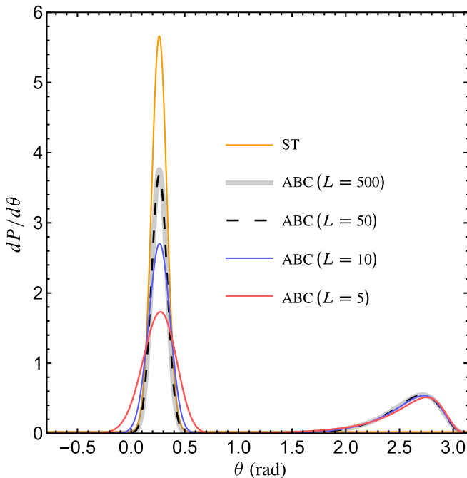
FIG. 7. Angular variation of the differential detection probability for a two-dimensional Gaussian wave packet of central momentum \mathbf{k}_0 = 9.66\hat{e}_x + 2.59\hat{e}_y approaching the L-shaped surface S . The colored curves represent the results from the ABC proposal for \beta = 2.59i at various finite detector distances (indicated in the legend). The ABC curves show minimal variation beyond L = 50 , and each one presents two distinct peaks, unlike the single peak predicted by ST (orange curve).
