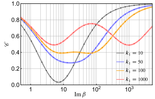
FIG. 2. ABC-ST contrast ( \mathcal{C}_\infty ) curves for the superposition of Gaussian wave packets Eq. (19), with \text{Re}\beta = 0 , k_0 = 5 , and a fixed k_1 (denoted in the legend). Plot markers indicate \mathcal{C}_L values for L = 10 , calculated using Eqs. (9), (6), and (20). Thick curves depict contrasts calculated from Eq. (21).
