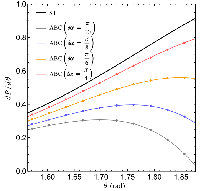
FIG. 5. Angular variation of the differential detection probability for a two-dimensional Gaussian wave packet of central momentum \mathbf{k}_0 = \sqrt{3} \hat{e}_y - \hat{e}_x approaching the inclined screen \mathcal{S}_\alpha . The black curve shows the \alpha -independent ST prediction, while colored curves represent predictions of the ABC proposal for \beta = 2i and different tilt angles \alpha = \pi/2 + \delta\alpha (see legend). Plot markers indicate numerical values derived from Eq. (26) for a finite detector distance of L = 15 .
