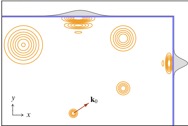
FIG. 6. A selection of contour plots illustrating the development of (34) over time. A wave packet approaching an L-shaped ABC screen generates screen-position probability distribution functions with two distinct peaks: the first peak, which would also be present for a flat screen, and the second peak, resulting from the portion of the wave packet that is reflected.
