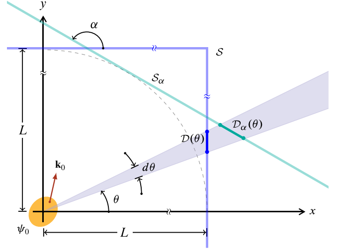
FIG. 4. A wave packet \psi_0 with mean momentum \mathbf{k}_0 approaches either an L-shaped screen S or a flat screen S_\alpha tilted at angle \alpha relative to the x axis. The infinitesimal detector segments \mathcal{D}(\theta) \subset S and \mathcal{D}_\alpha(\theta) \subset S_\alpha both span the same convex cone of apex angle d\theta (shaded area).
