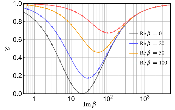
FIG. 1. ABC-ST contrast ( \mathcal{C}_\infty ) curves for the Gaussian wave packet (13) with k_0 = 20 and a fixed \text{Re}\beta (denoted in the legend). The plot markers indicate \mathcal{C}_L values for L = 2 , calculated from Eqs. (9) and (6) using the time-dependent wave packet \psi_t^G(x; k_0, \beta, L) , Eq. (17).
