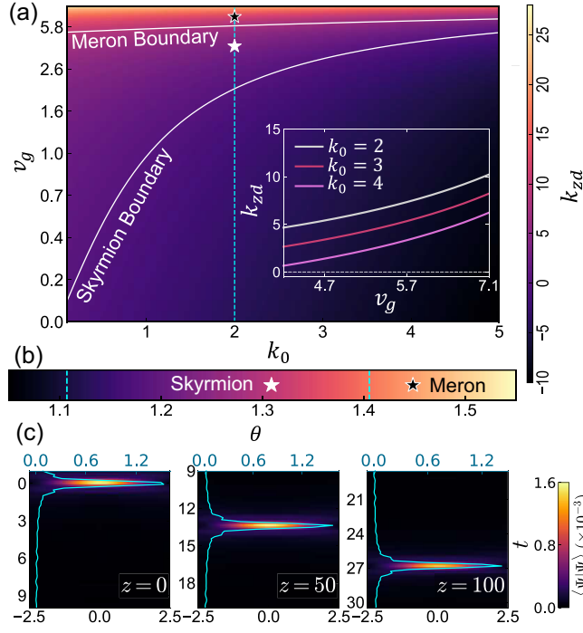
FIG. 2. (a) The allowed parameter space in v_g, k_0 to host skyrmion and meron in momentum space in an electron STWP. The colormap is the longitudinal spectral linewidth in momentum space, and the white and black stars are the points used for skyrmion and meron real-space calculations, respectively. Inset: The longitudinal spectral linewidth as a function of group velocity and carrier wave numbers. The shown k_{zd} is measured without a limit k_{z\max} . (b) The group velocity regions for a carrier wave number of k_0 = 2 , shown using the spectral tilt angle. (c) The propagation invariance of the electron STWP can be seen by the almost unchanged peak intensity (blue line and axis) as the pulse moves from z = 0 to z = 100 . The probability amplitude plot is scaled by 10^3 for clarity, and shown in the laboratory frame.
