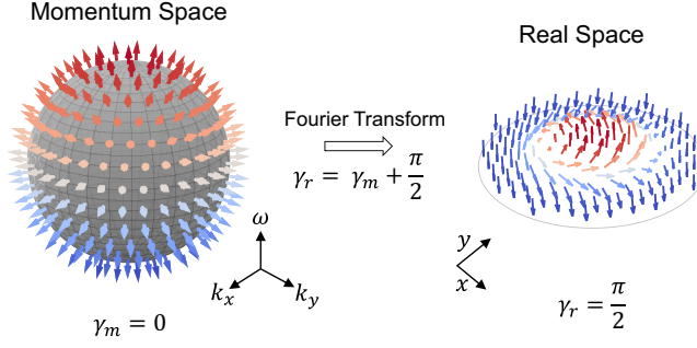
FIG. 4. The relation between the 3D Skymiononic spinor texture in momentum space and its in-plane Fourier transformed counterpart in real space. There is a helicity shift of \pi/2 due to an extra i^m term, with m = 1 being the winding number (see Sec. B of the Supplemental Material [14]). \gamma_m is the helicity in momentum space of the spinor texture and \gamma_r is the real-space helicity.
