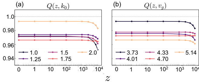
FIG. 5. (a) The propagation invariance of the skyrmion SEV for group velocity of v_g = 3.73 for different carrier wave numbers, and (b) the propagation invariance of the skyrmion SEV as a function of the group velocity, for k_0 = 2.0 .
