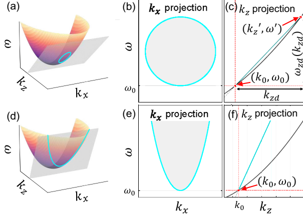
FIG. 1. (a) The construction of momentum space skyrmion uses a closed spectral loop in (b) k_x - \omega space. (c) The intersection of the spectral plane and the dispersion surface gives the lowest point (k_0, \omega_0) called the carrier, and the point (k'_z, \omega') . The difference between them is k_{zd} . When \omega' is the maximum allowed constituent electron plane wave energy, we write the point as (k_{z\max}, \omega_{\max}) in text. (d)–(f) Merons can be obtained from an intersection that produces a parabolic projection in the k_x - \omega plane instead.
