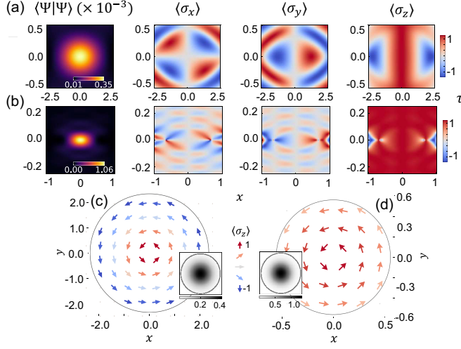
FIG. 3. The real-space structure of the electron wavefunction. (a), (b) The spatiotemporal structure for skyrmions and meron SEV, respectively, in the comoving frame. The SEV is normalized by the local probability amplitude. (c) The real-space SEV of the skyrmions and (d) merons. The in-plane arrows are directions of \langle\sigma_x\rangle and \langle\sigma_y\rangle , while the colormap and legend gives the direction of \langle\sigma_z\rangle . Inset: Probability map of the electron pulse with the skyrmion and meron structure embedded, scaled to 10^3 .
