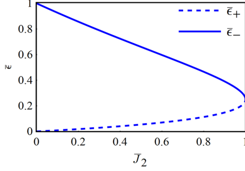
FIG. 4. The normalized COP is plotted as a function of the normalized cooling power. The dashed and solid curves represent the \bar{\epsilon}_+ (positive root) and \bar{\epsilon}_- (negative root) of Eq. (A6), respectively. Here, we set \epsilon_C^T = 1 .
