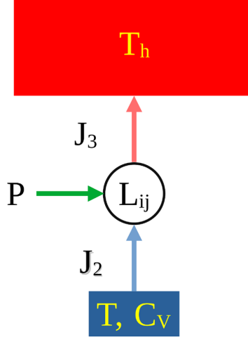
FIG. 1. The schematic diagram of a minimally nonlinear irreversible refrigerator working with a finite-sized cold heat bath and an infinite-sized hot heat bath.
