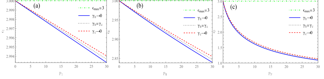
FIG. 2. The COP of the refrigerator is plotted as a function of average input power: for an ideal gas cold heat bath [panel (a)], for degenerate electronic gas cold heat bath [panel (b)], and for phonon gas cold bath at low temperature [panel (c)]. The green dot-dashed line indicates \epsilon_{\max} = 3 . The solid blue curve represents the lower asymmetric dissipation limit, \gamma_h \rightarrow 0 ( \gamma \rightarrow 1 ) [Eq. (32)]. The dotted black curve represents the symmetric dissipation case \gamma_h = \gamma_c ( \gamma = 2 ) [Eq. (34)]. The dashed red curve represents the upper asymmetric dissipation limit, \gamma_c \rightarrow 0 ( \gamma \rightarrow \infty ) [Eq. (33)]. We set following values: E = 50 and -\Delta U = \epsilon_{\max} E [from Eq. (31)].
