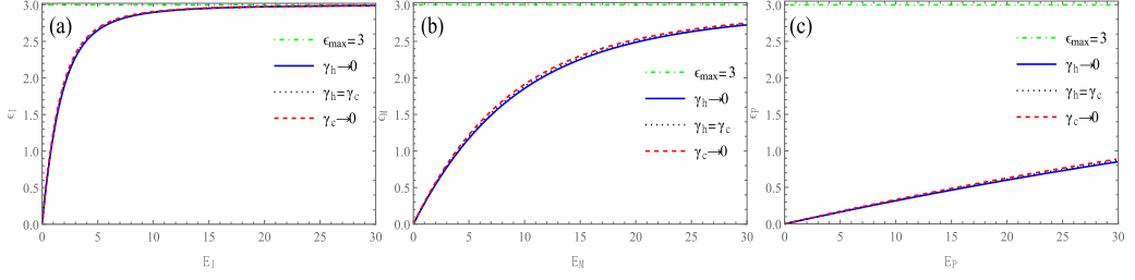
FIG. 3. The COP of the refrigerator is plotted as a function of exergy: for an ideal gas cold heat bath [panel (a)], for degenerate electronic gas cold bath [panel (b)], and for phonon gas cold heat bath at low temperature [panel (c)]. The green dot-dashed line indicates \epsilon_{\max} = 3 . The solid blue curve represents the lower asymmetric dissipation limit, \gamma_h \rightarrow 0 ( \gamma \rightarrow 1 ) [Eq. (32)]. The dotted black curve represents the symmetric dissipation case, \gamma_h = \gamma_c ( \gamma = 2 ) [Eq. (34)]. The dashed red curve represents the upper asymmetric dissipation limit, \gamma_c \rightarrow 0 ( \gamma \rightarrow \infty ) [Eq. (33)]. We set the following values: P = 20 and -\Delta U = \epsilon_{\max} E .
