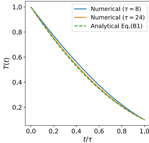
FIG. 5. Comparison between numerical and analytical results of T(t) for \tau = 8 and \tau = 24 . We used T_i = T_h = 1 and T_f = 0.1 .
